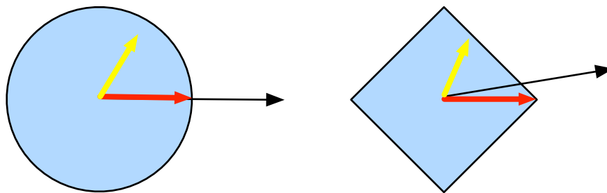
图11.2.4: Convex Projections.
